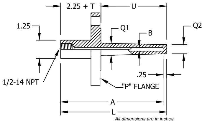
Tapered Shank
