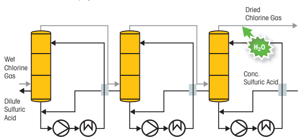
Conventional Chlorine Drying
