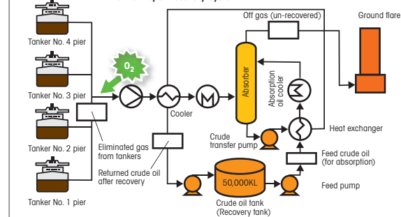
Process flow diagram of Tanker Vapor Recovery System
