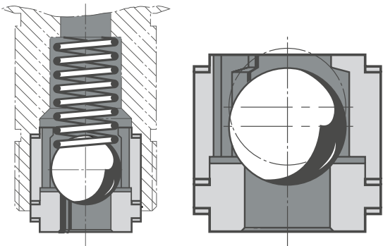
Ball valve
