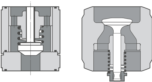
Cone valve
