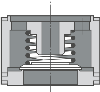
Disc valve
